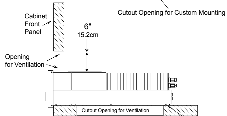
MA5200 Side View in Custom Cabinet
